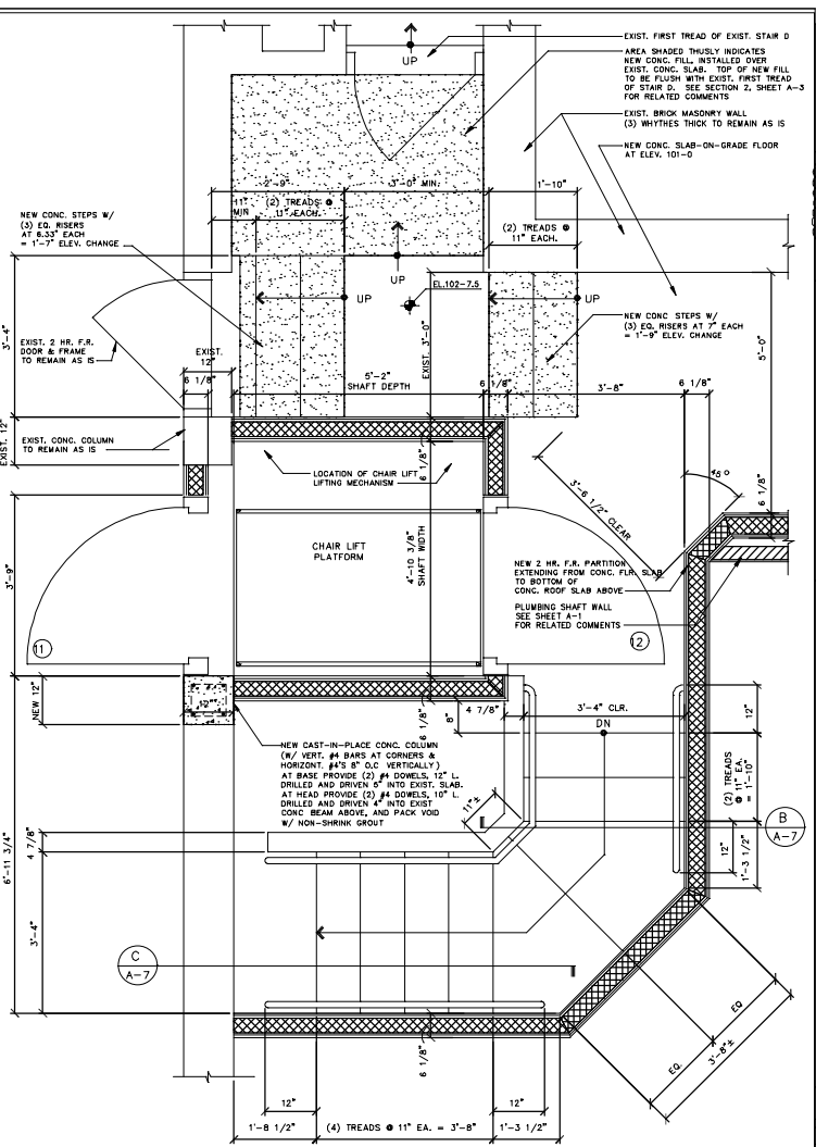
D PLAN DETAIL AT CHAIR LIFT (AT UPPER GARAGE & INTERN. LANDING)
