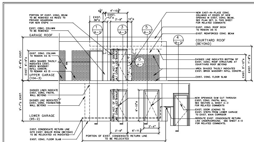
A INTERIOR ELEVATION AT NORTH GARAGE WALL
