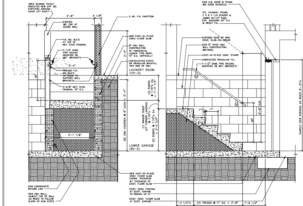
B SECTION AT STAIR TO LOWER GARAGE
