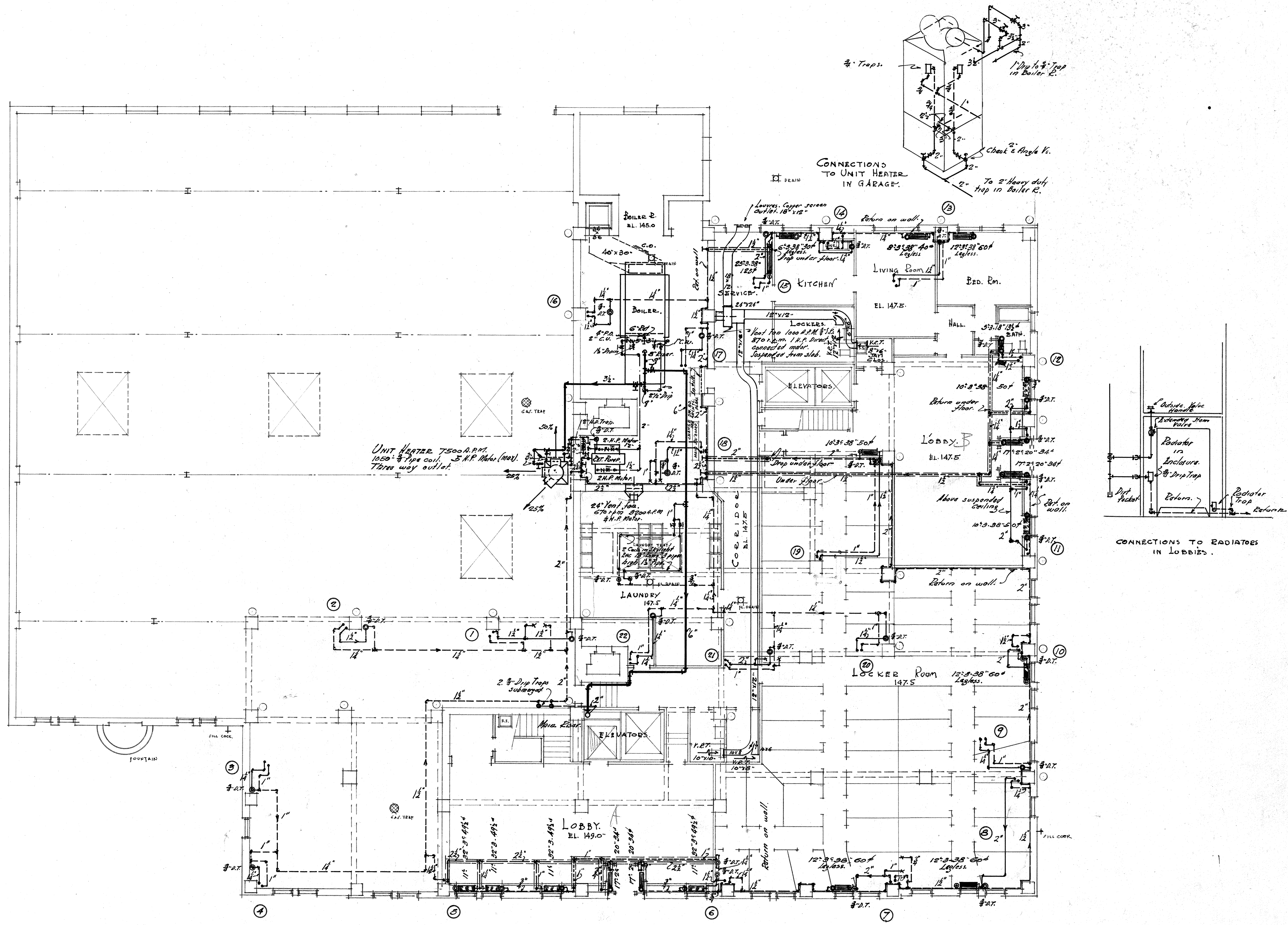
GROUND (FIRST) FLOOR PLAN.
