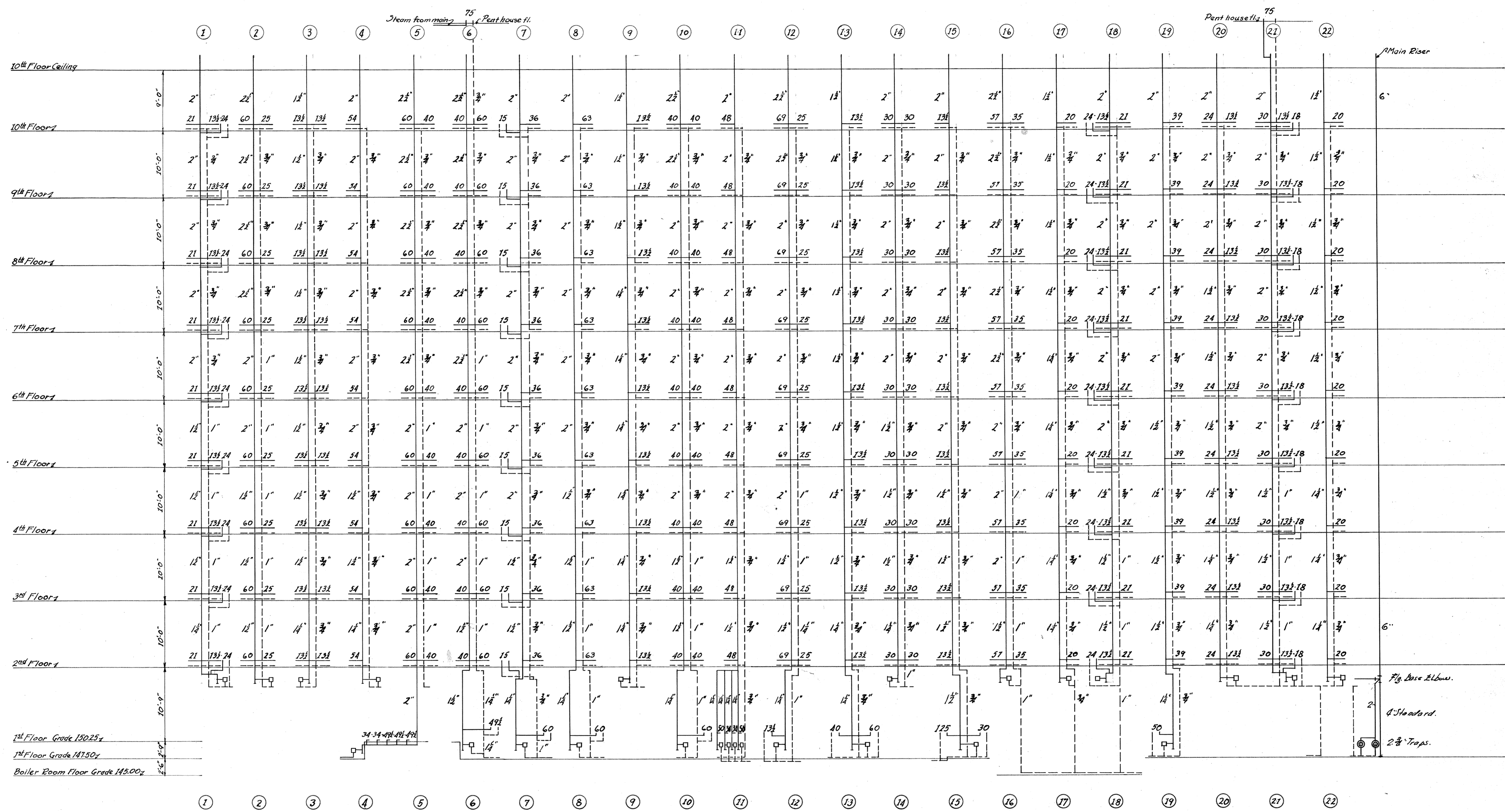
RISER DIAGRAM. ANCHOR ALL RISERS EXCEPT MAIN RISER AT 6 th FLOOR.
